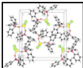
Fig. 2. Crystal packing, viewed down a axis, of the title compound.
